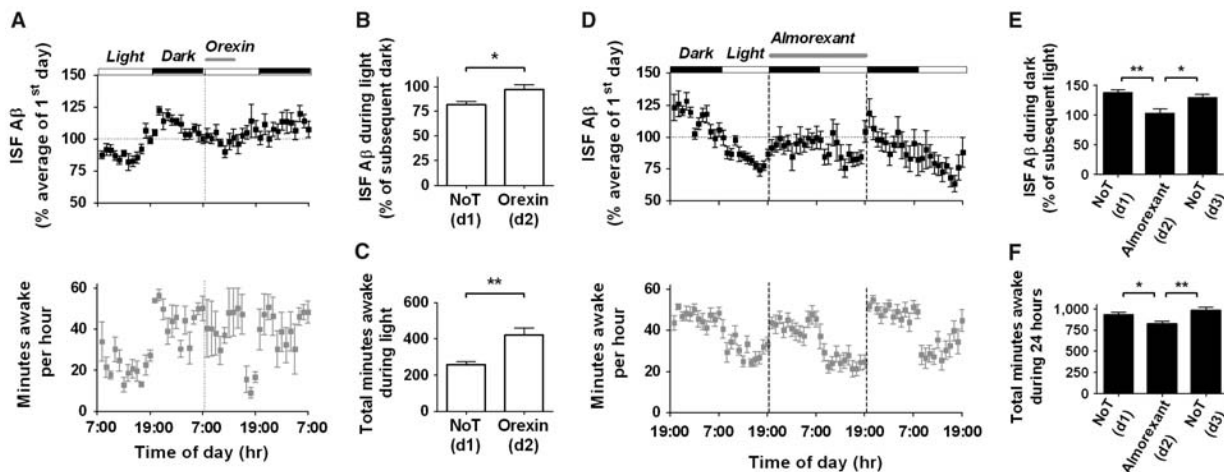
Fig. 3. Effects of orexin and a dual orexin receptor antagonist on ISF Aβ levels in Tg2576 mice. (A) After 24 hours of baseline measurement, orexin (1.5 pmol/hour) was infused icv for 6 hours at the beginning of the light period. This sustained ISF Aβ levels from the dark period and kept the mice awake longer. (B and C) Infusion with orexin increased Aβ levels during the light period and thereby abolished the normal 20% difference between the dark and light period ( *P = 0.01 , n = 7 ). Orexin increased the time spent awake by 163 min ( **P = 0.009 , n = 5 ), compared to that during the light period 24 hours previously. (D) After 24 hours of baseline
